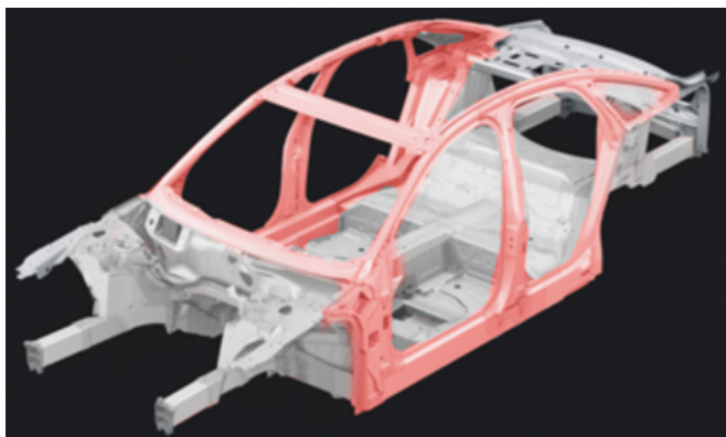
DRAWING SP body:
